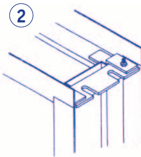
HEAD JAMB CONNECTION
