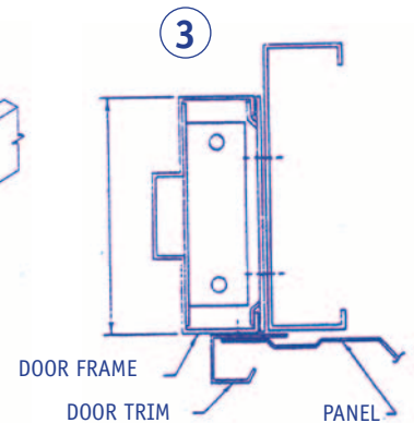
SUB JAMB CONNECTION
