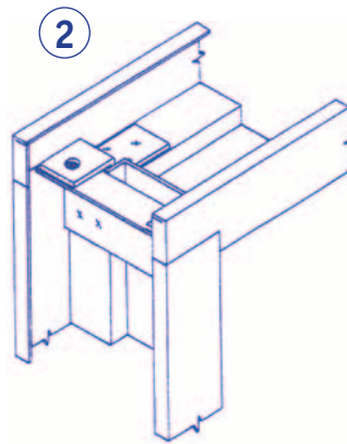
HEAD/JAMB CONNECTION
